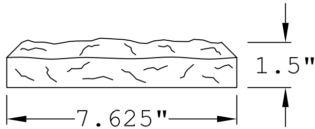
SIDE/END VIEW
